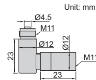
90° ADAPTER Code 4653-K1
